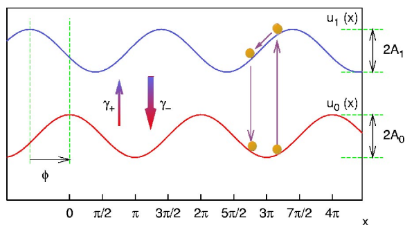
FIG. 1. (Color online) Diagram of the system considered in this work. A Brownian particle can live in two different internal states 0 and 1 corresponding to \phi -shifted potentials; the transition rates are asymmetric ( \gamma_+ \neq \gamma_- ). The rectification process is shown in the right-hand side of the figure (see text).
