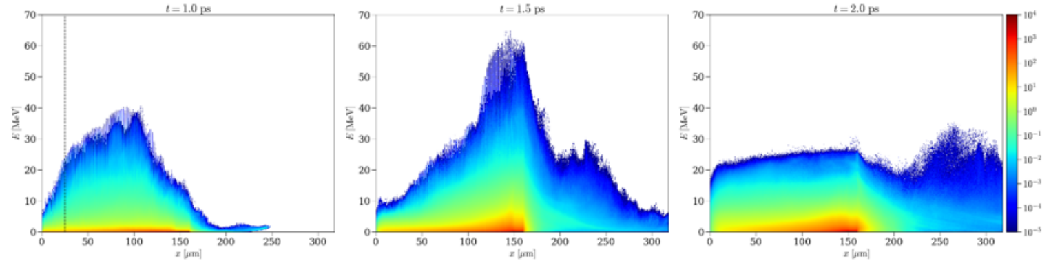
spatially resolved energy distribution of electrons
