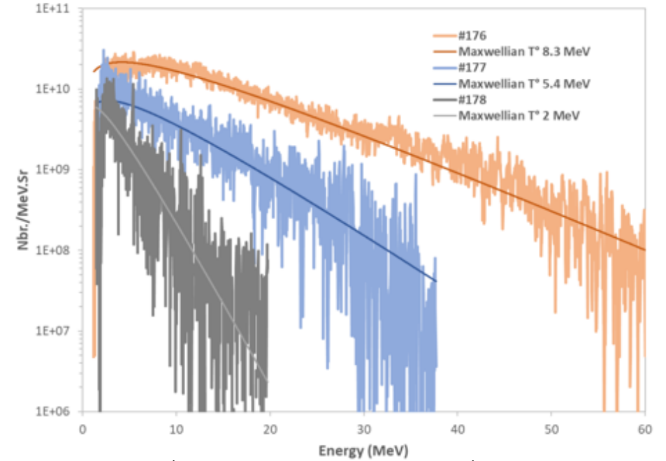
Electrons energy spectra measured at 13.5°
